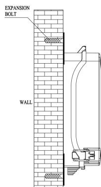
Wall Mount
