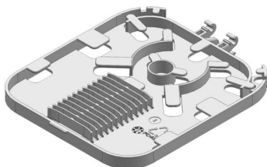
12 Fibers/Tray Suitable for 1×8 Micro PLC Splitter
